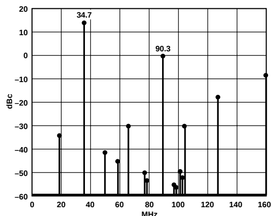
Figure 5. Typical DDS Output Spurious Performance
