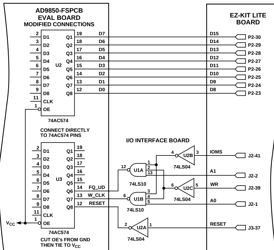
Figure 2. Schematic of I/O Decode Logic and Interconnections
