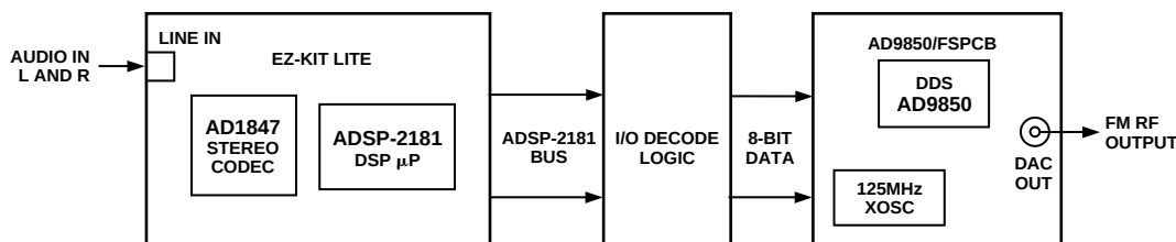
Figure 1. Block Diagram of FM RF Generator Implementation
